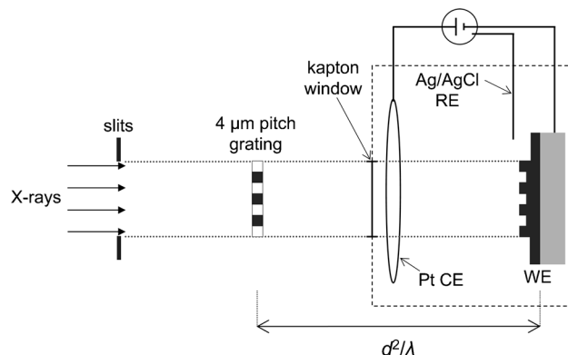
Figure 1. Conceptual plan for electrochemical X-ray photolithography.
